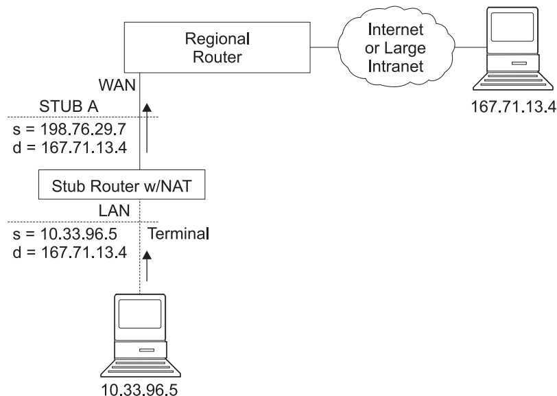
Figure 45. Network Running NAT
