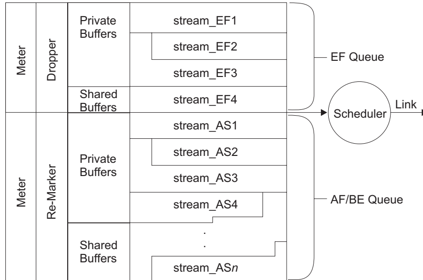
Figure 40. Relationship of Policar, Buffers, Queues, and Scheduler
