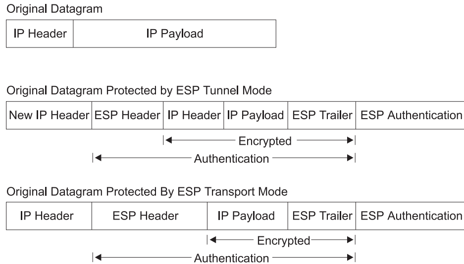
Figure 35. ESP-Protected Datagram Format
