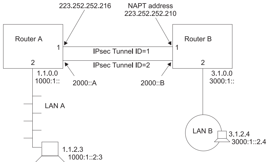
Figure 38. Network with IPsec and NAT
