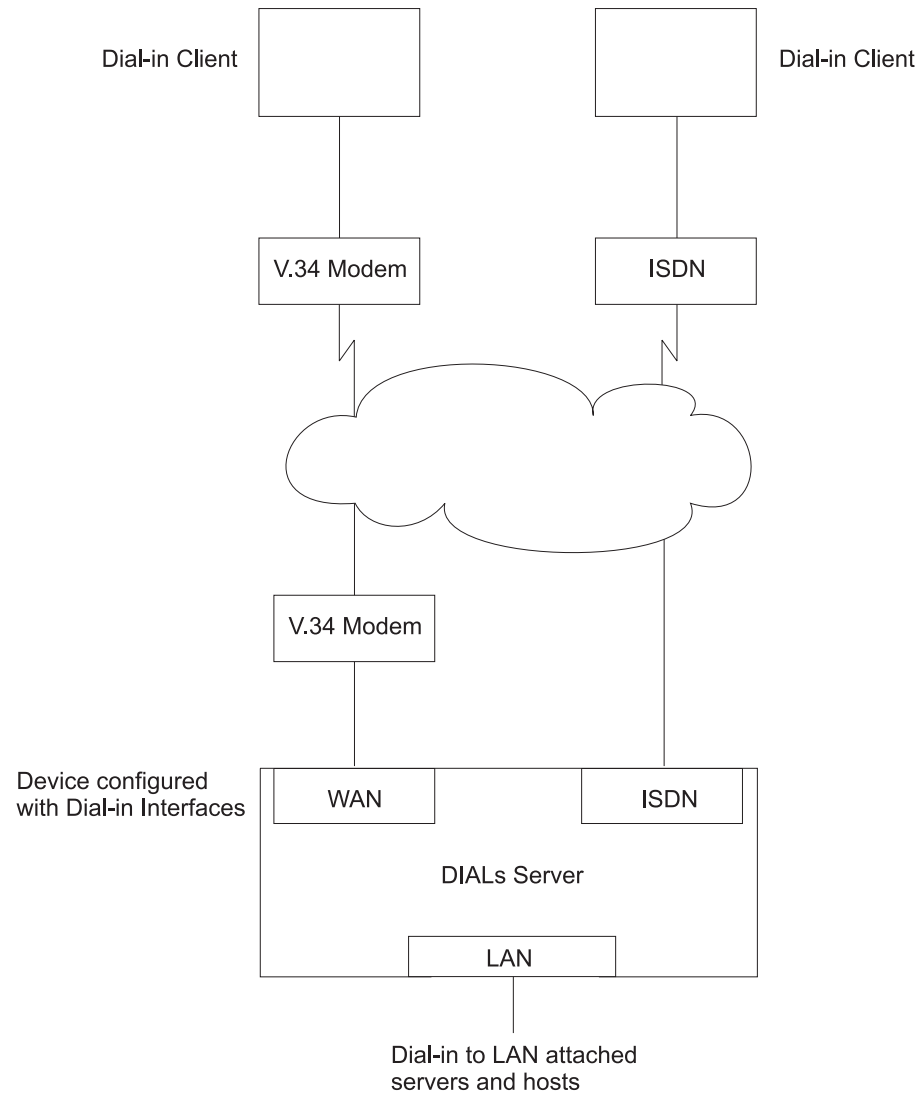
Figure 46. An Example of a DIALs Server Supporting Dial-In
