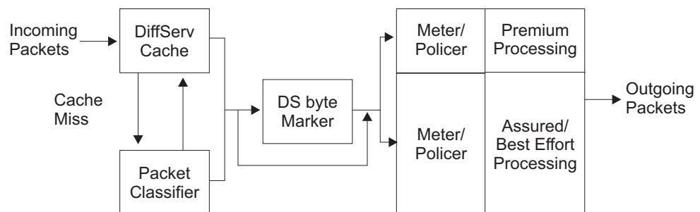
Figure 39. DiffServ Data Packet Path
