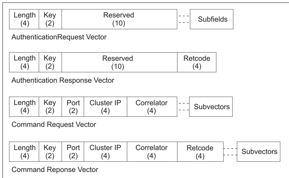
Figure 18. Command Response Vector
