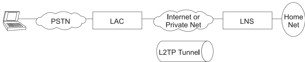
Figure 43. Sample L2TP Network
