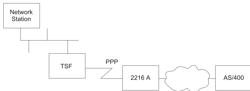
Figure 51. TSF Sample Configuration
