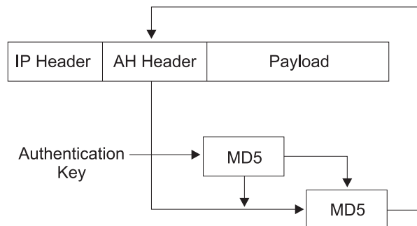
Figure 33. Creation of an HMAC MD5-Authenticated Message
