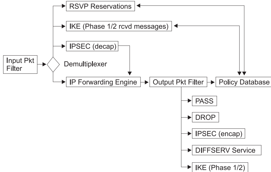
Figure 27. IP Packet Flow and the Policy Database
