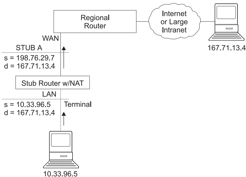
Figure 44. Network Running NAT
